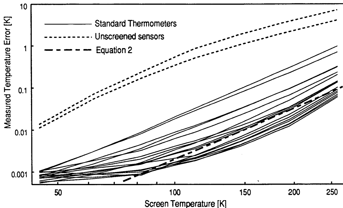
Figure 5. Measured temperature deviation when exposing the thermometers to photon radiation. The total number of thermometers investigated is 22. Two unprotected sensors are also shown and as expected they are much more sensitive to thermal radiation.
