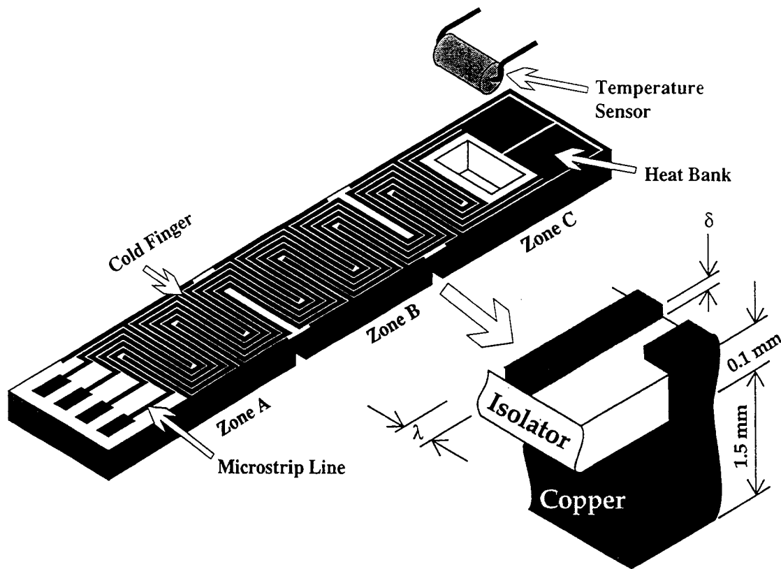
Figure 1. Thermometer layout showing the meandering microstrip lines of width \lambda and thickness \delta , the solid copper plate thickness corresponds to that of a standard Allen Bradley carbon sensor. The thermometer size is 100 mm x 10 mm x about 2 mm.
