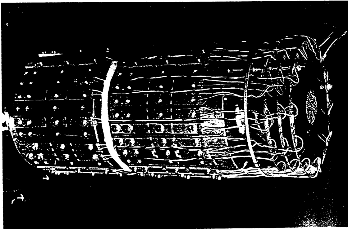
Figure 3. Photograph of the validation insert. The size of the thermometers is 100 mm x 10 mm x 2 mm and about a dozen thermometers can be seen bolted to the isothermal copper substrate. The wire terminal heaters are on the right-side. The heat radiation shield is removed. Liquid helium is present inside a cavity enclosed by the copper substrate
