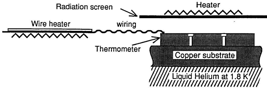
Figure 2. Schematic principle of the thermometer validation system. The thermometers are bolted to an isothermal substrate. The vacuum, the temperature of the electrical leads and the radiation screen can be regulated.
